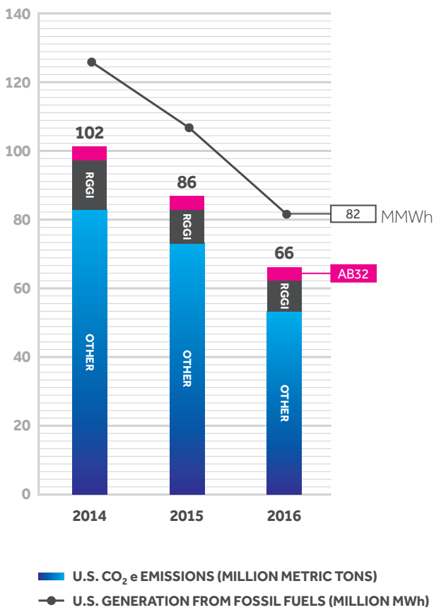
U.S. CO 2 e emissions and generation
