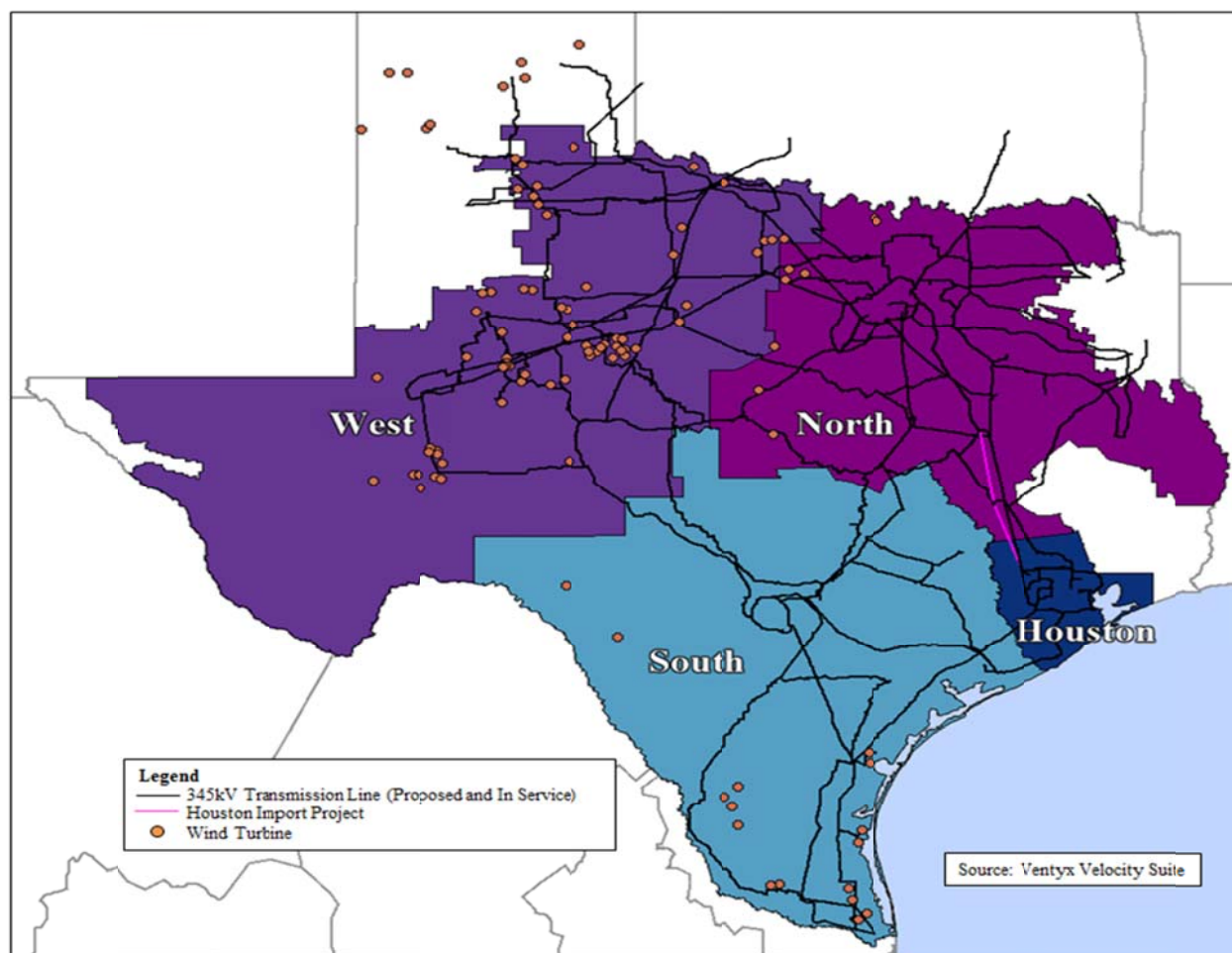
Figure 7 ERCOT Wind Turbines and 345 kV Transmission Lines
